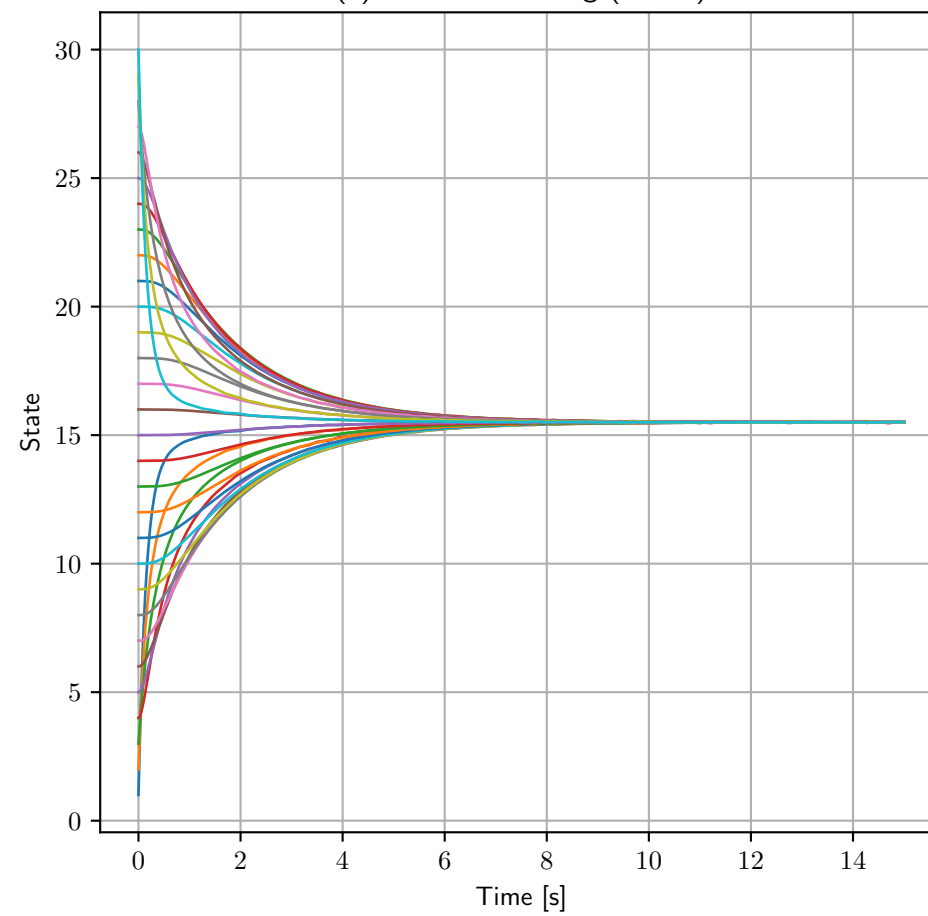
(e) Consensus: Ring ( k = 2 )
