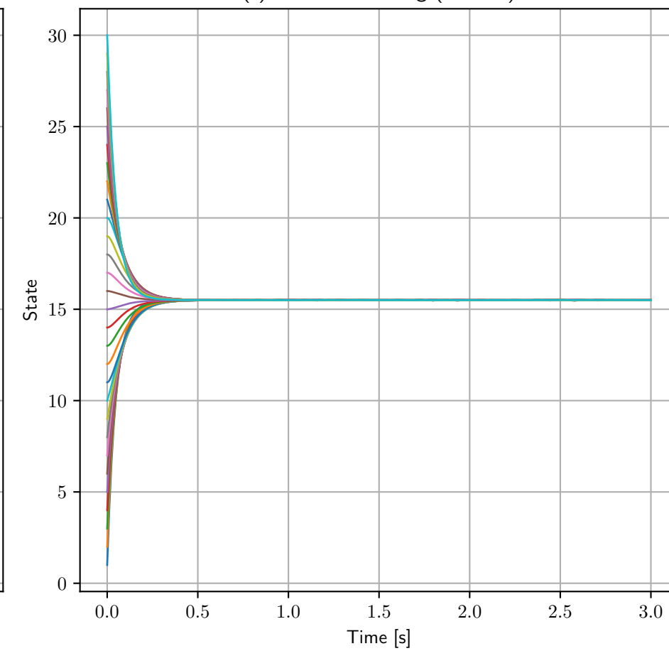
(f) Consensus: Ring ( k = 10 )
